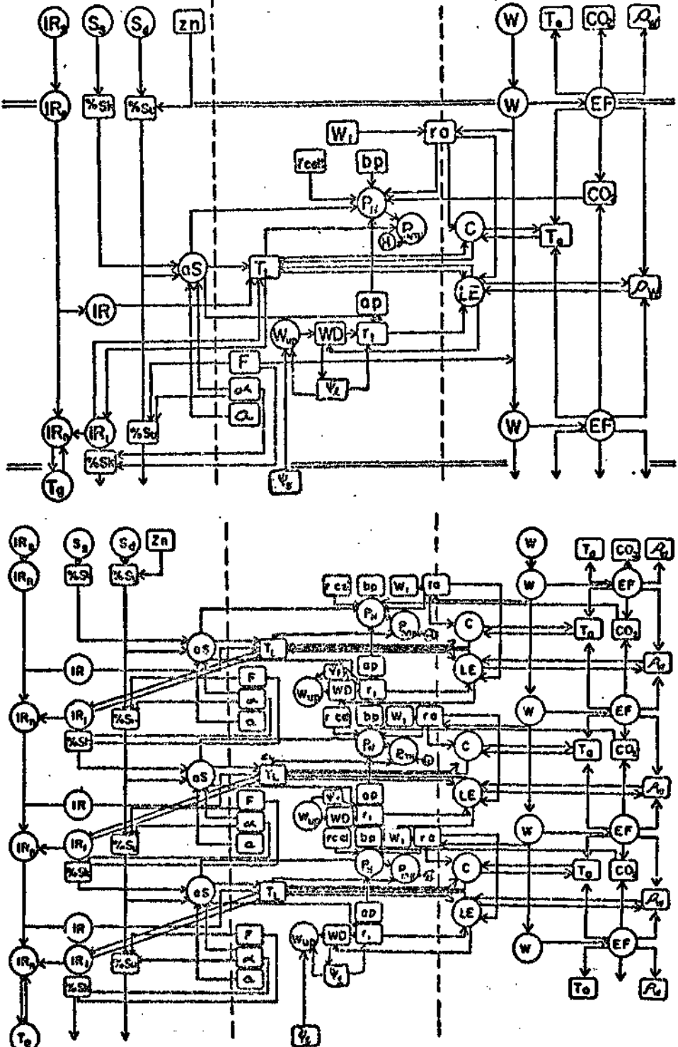
Fig. 1. Flow charts illustrating the interrelations between canopy variables and physical processes. Symbols are defined and explained in the text. The upper chart illustrates the interrelations for one level in the canopy; the lower chart, for a canopy divided into three levels. (after Miller, 1972)
