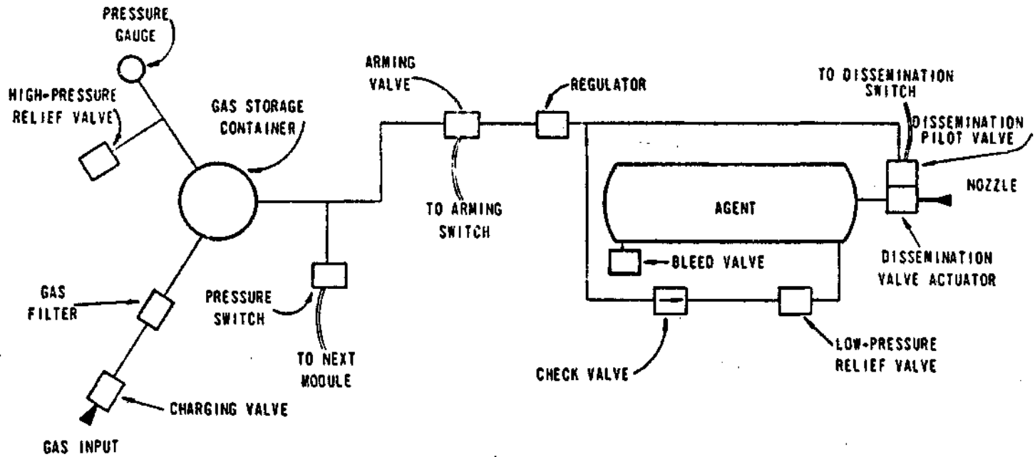
Figure 55. System Schematic
