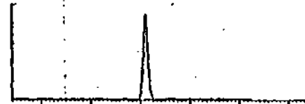
Figure 1. Mass chromatograms from a 10-g sample of pool L (1.6 ppt) showing separation between 2,3,7,8- and 1,2,3,4-TCDD.
