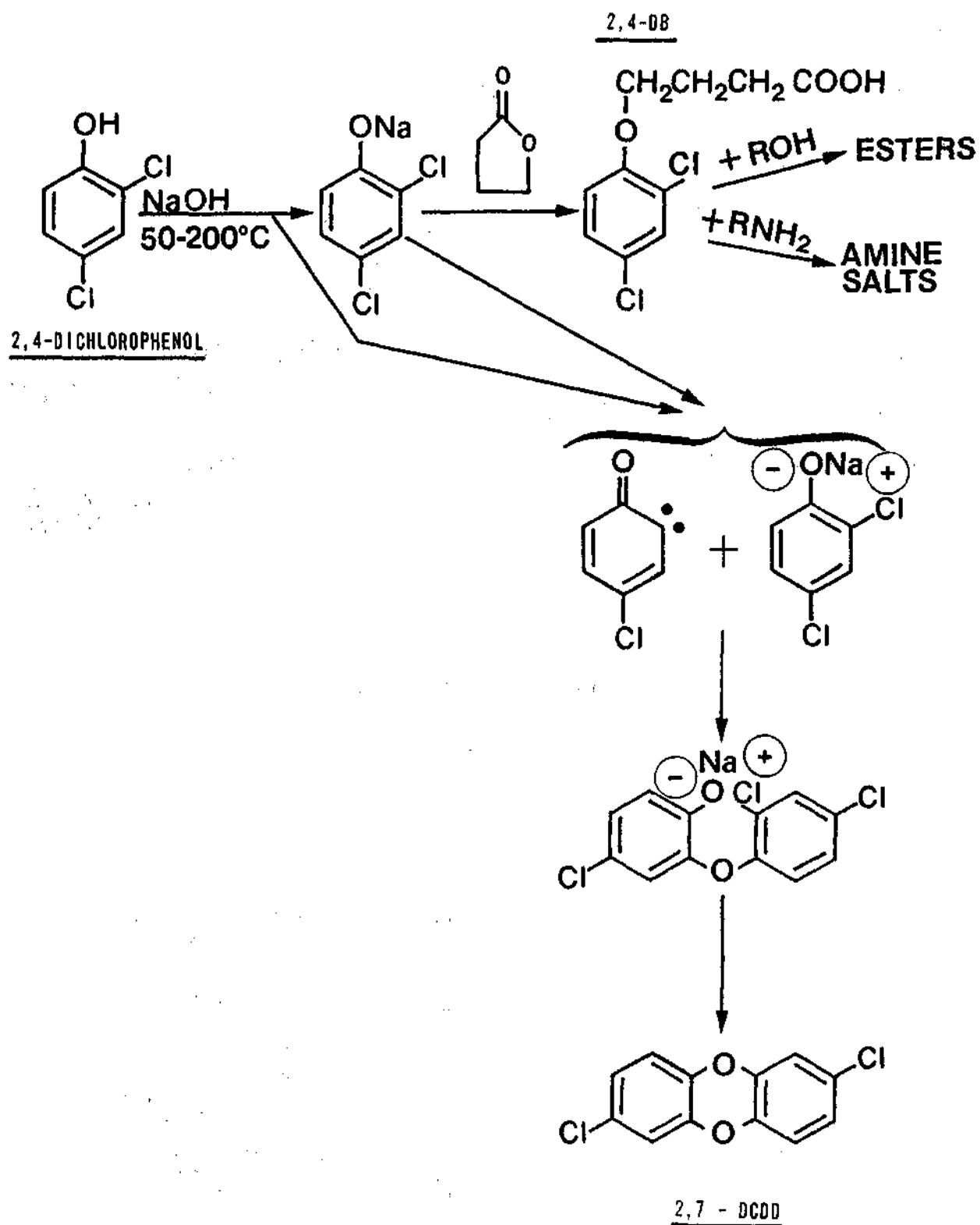
Figure 17. 2,4-DB.
