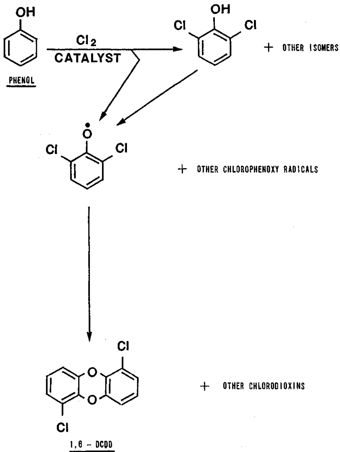
Figure 8. 2,6-Dichlorophenol.
