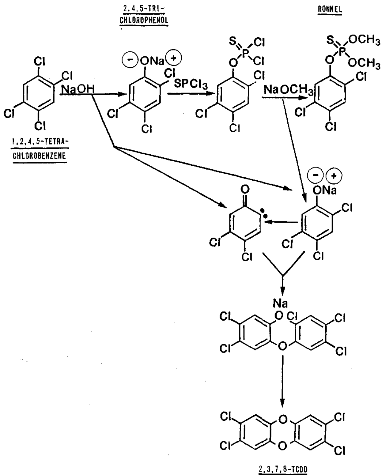
Figure 14. Ronnel.
