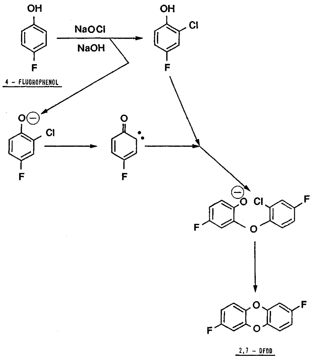
Figure 2. 2-Chloro-4-fluorophenol.
