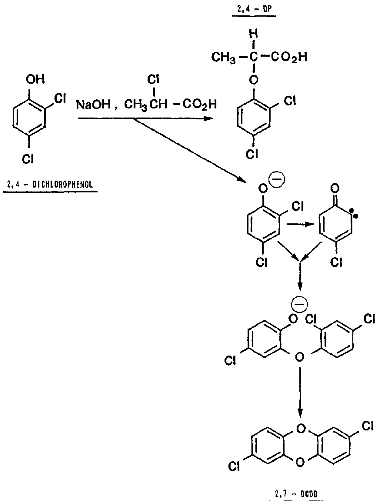
Figure 18. 2,4-DP.
