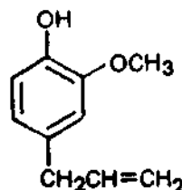
(27) EUGENOL
