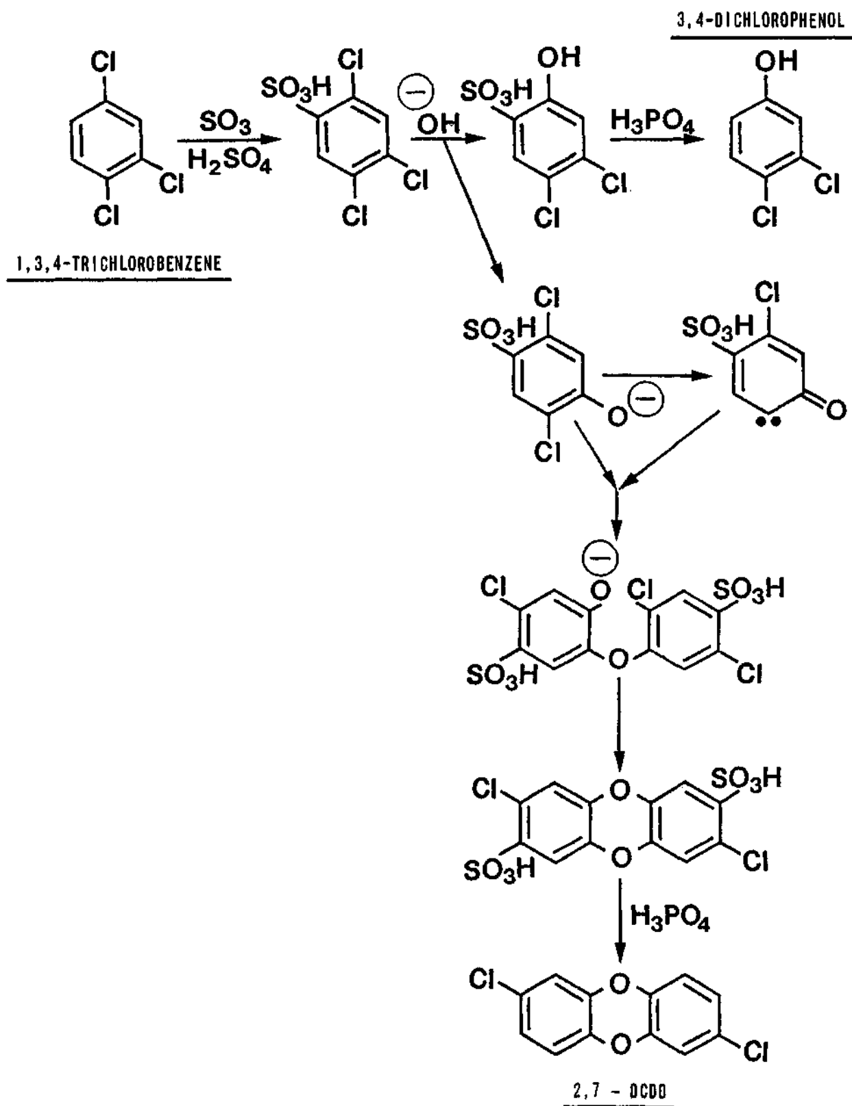
Figure 9. 3,4-Dichlorophenol.
