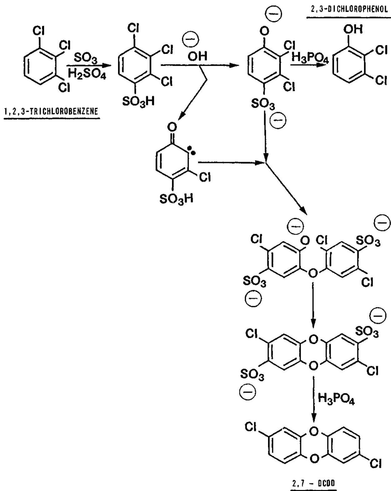
Figure 5. 2,3-Dichlorophenol.
